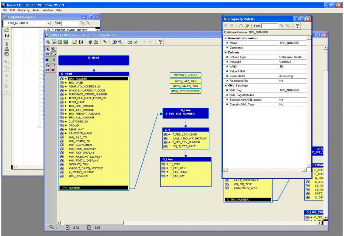
Sample 1: Reports Developer Tool
